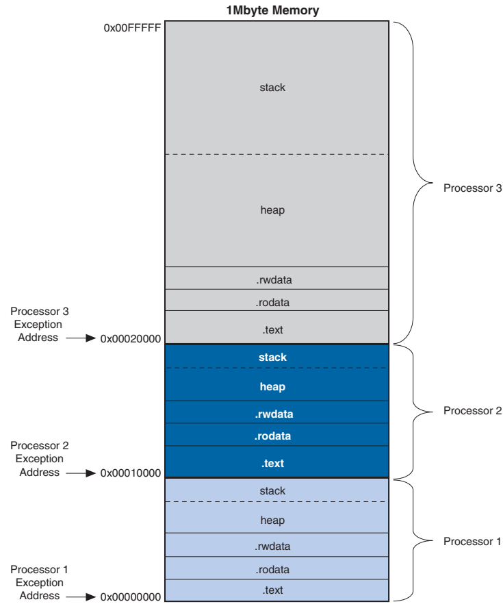
Figure 7: Partitioning of SDRAM Memory Map for Three Processors
