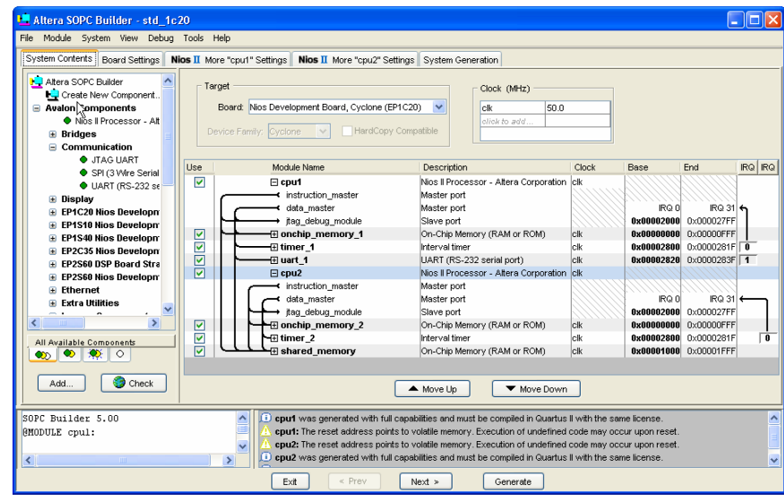
Figure 3: Multiprocessor System Sharing On-Chip Memory
