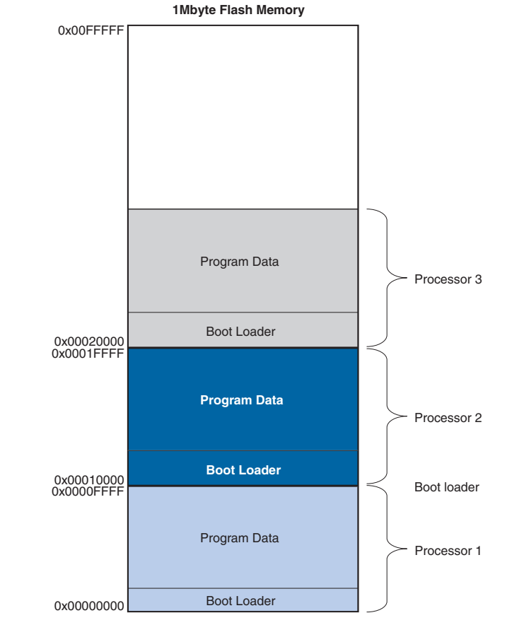
Figure 8: Flash Device Memory Map with Three Processors Booting
